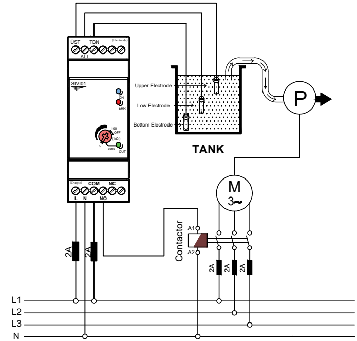
Connection Diagram for Draining the Tank
