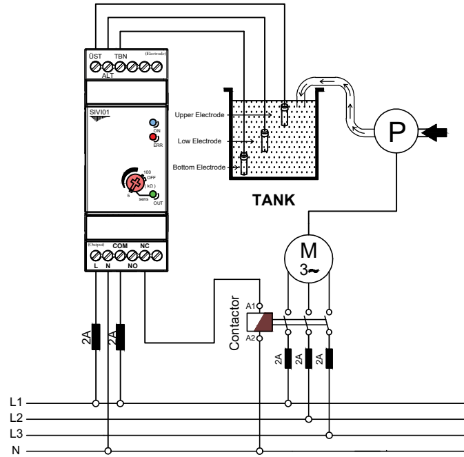
Connection Diagram for Filling the Tank
