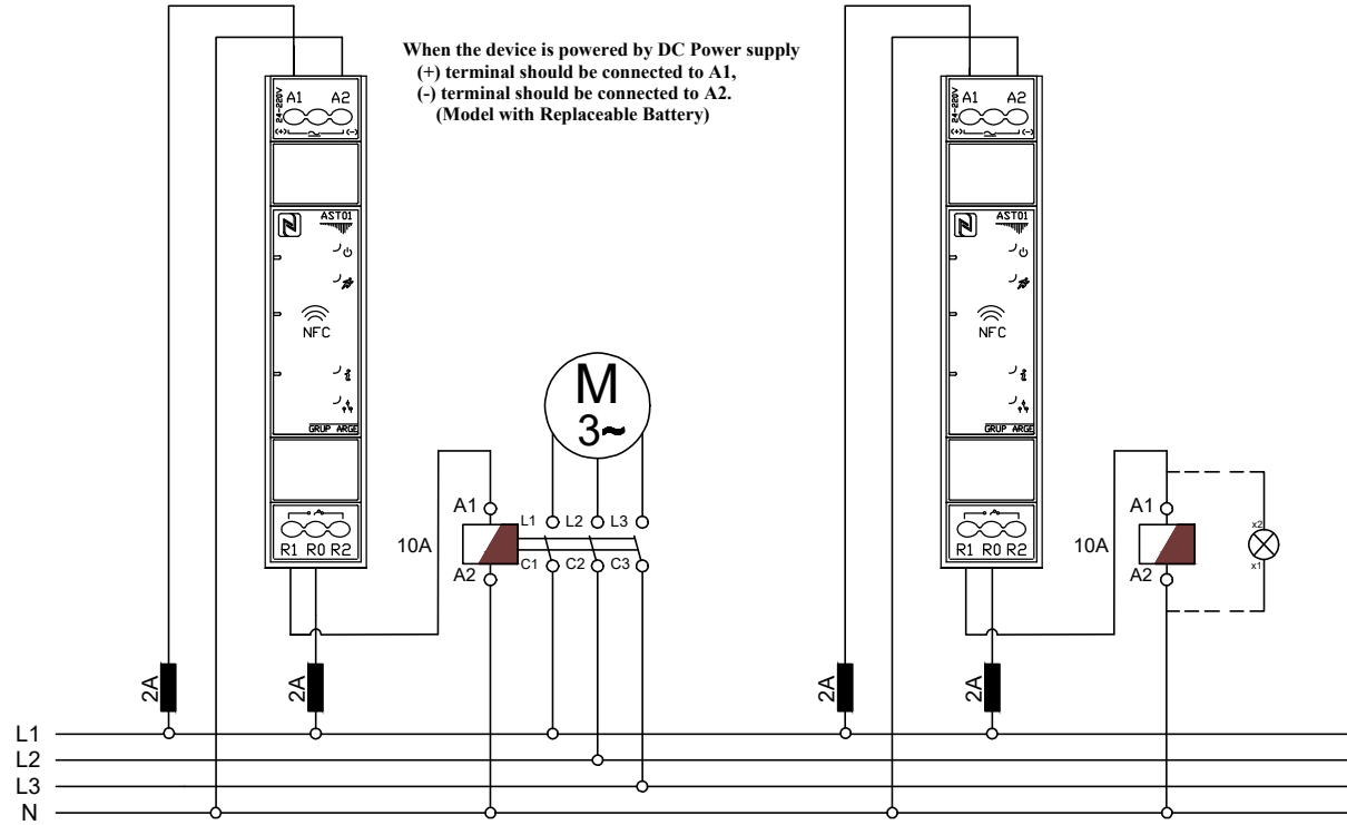
MONO-PHASE CONNECTION DIAGRAM
