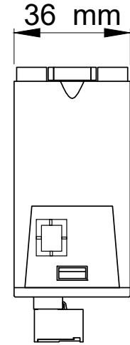
Top View
