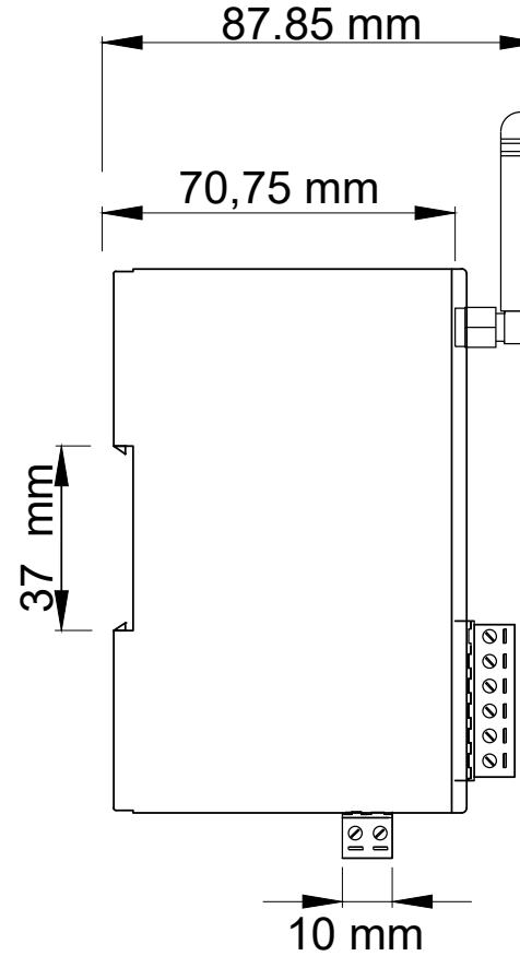
Side View
