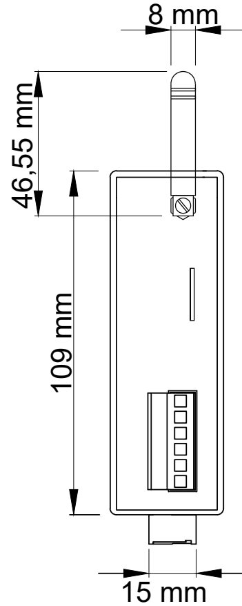
Bottom View
