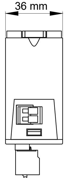
Top View
