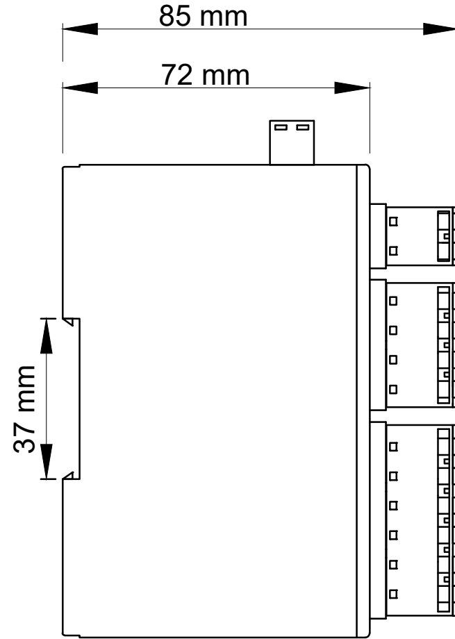
Side View
