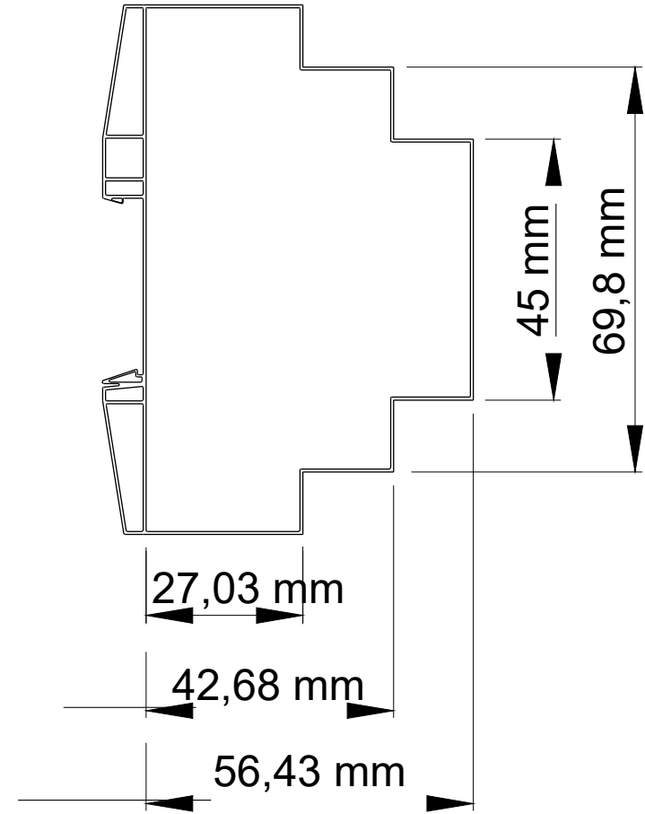
Side View
