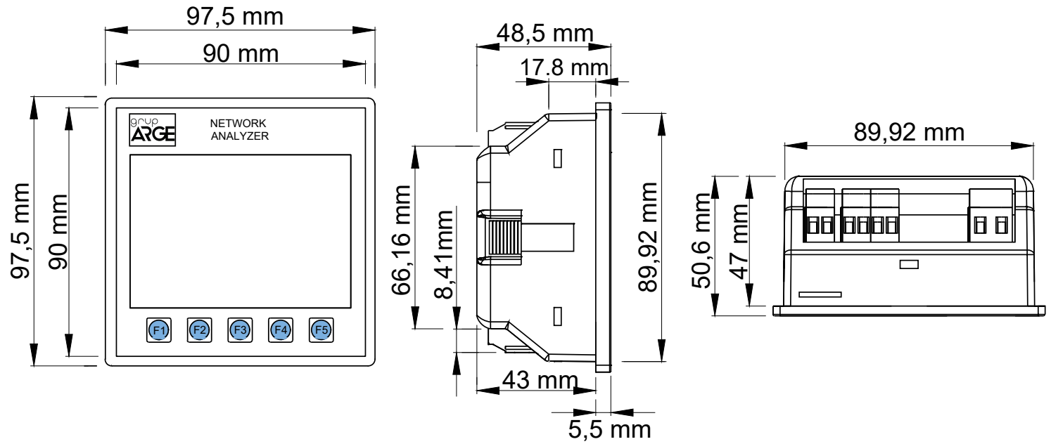
Front View
