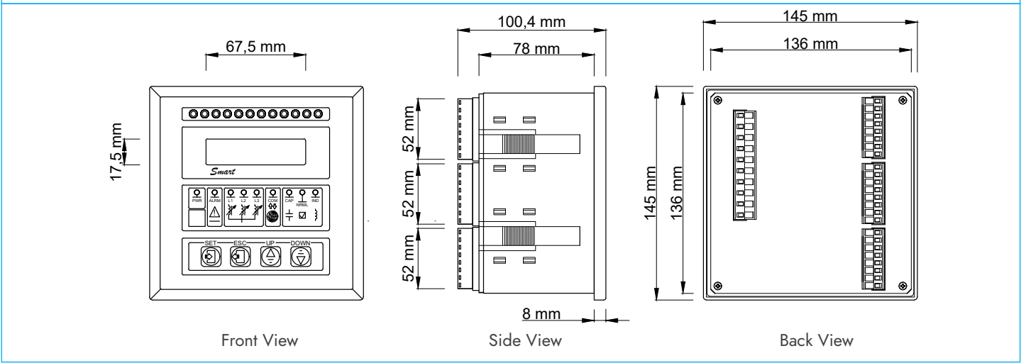
Smart S18-T and Smart 22-T Power Factor Controllers
