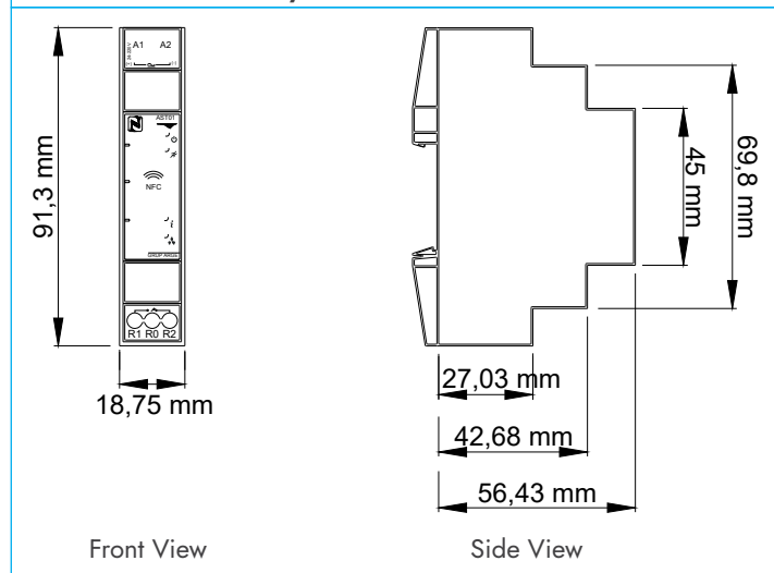
Astromomic Time Relay
