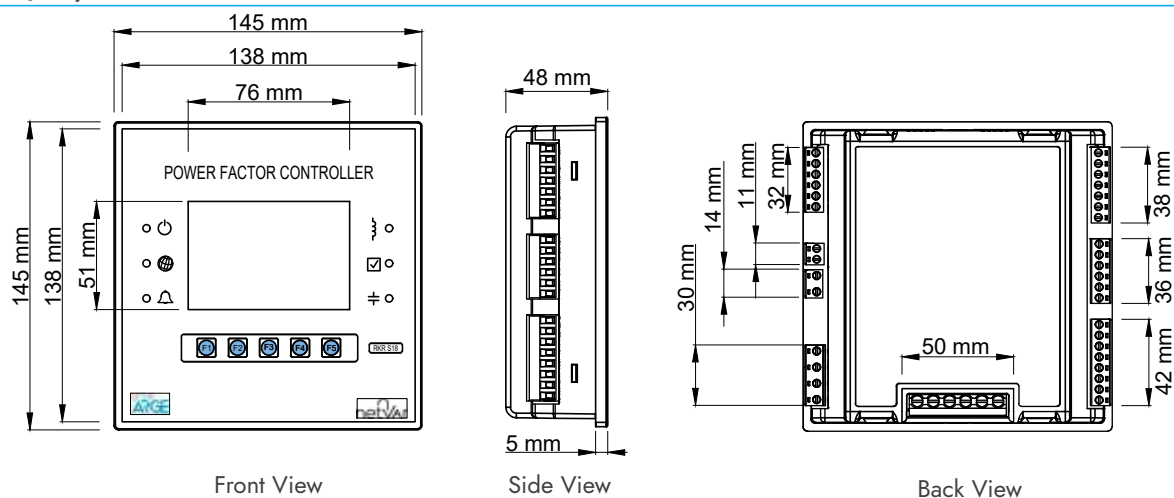
RKR S(12/18/24) SVC - Enabled Power Factor Controller
