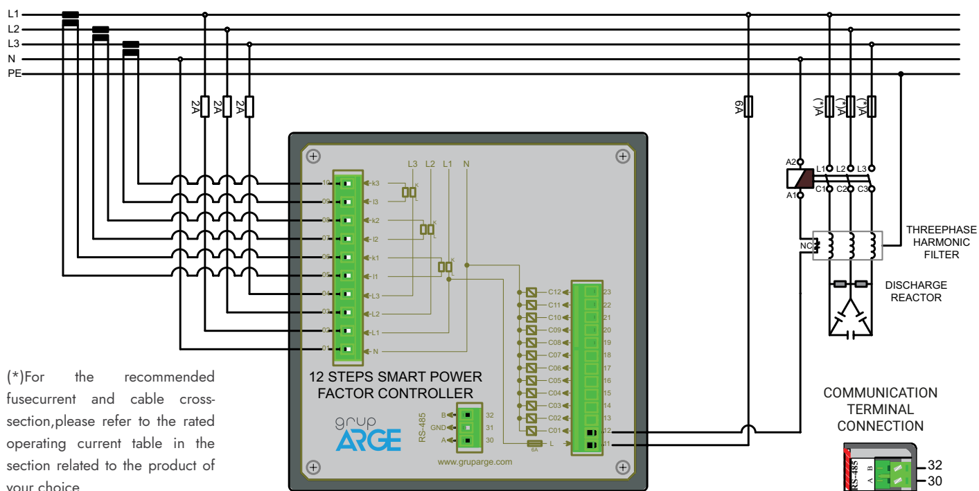
Smart 12 Power Factor Controller
