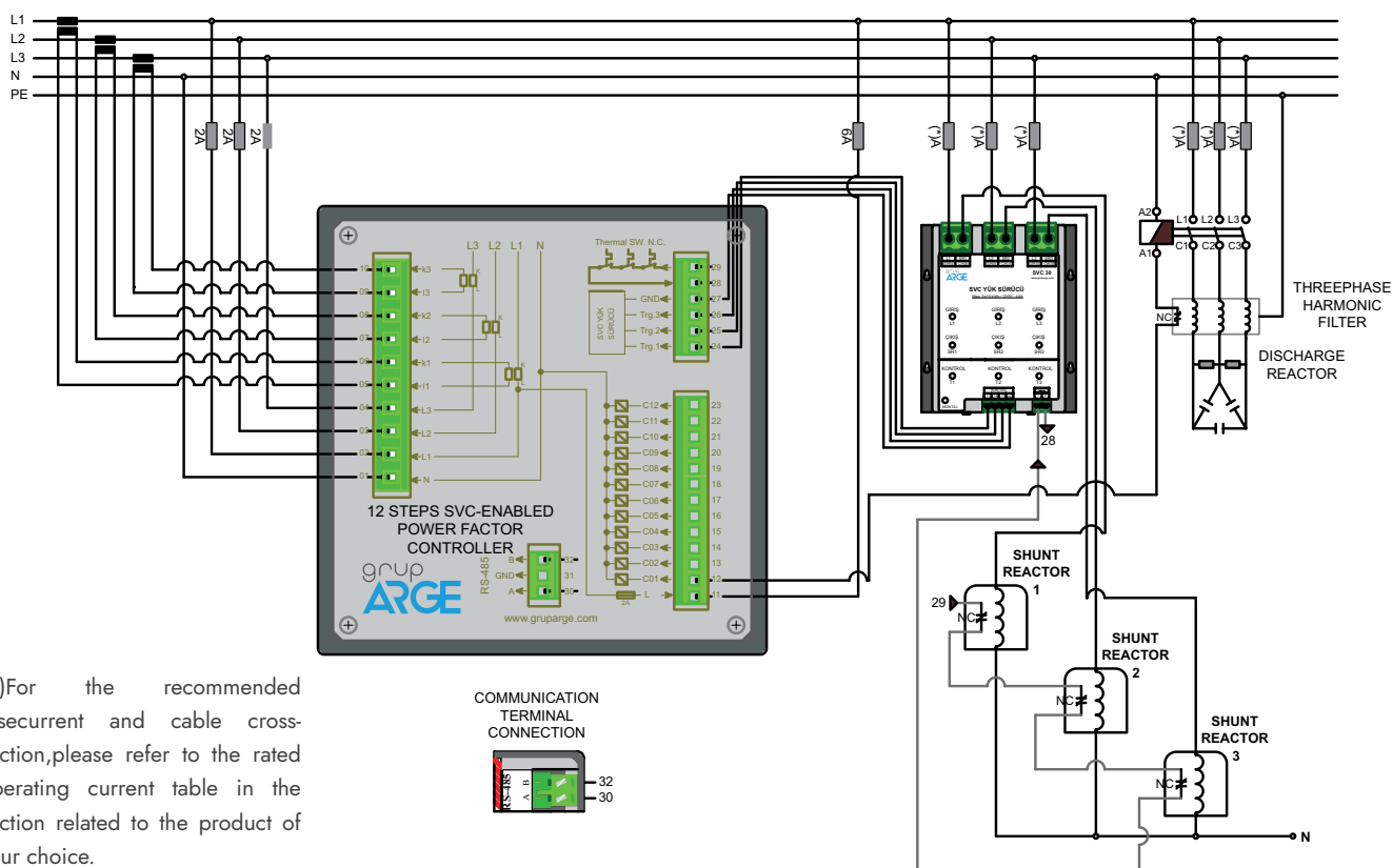
Smart S12 SVC - Enabled Power Factor Controller
