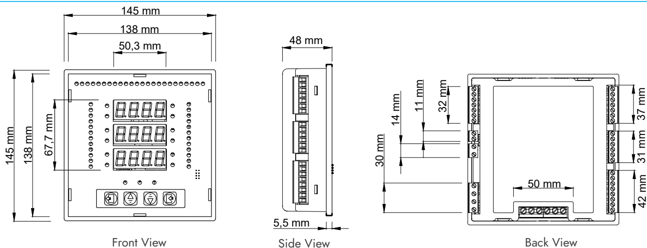
RKR (12/18/24) Power Factor Controller
