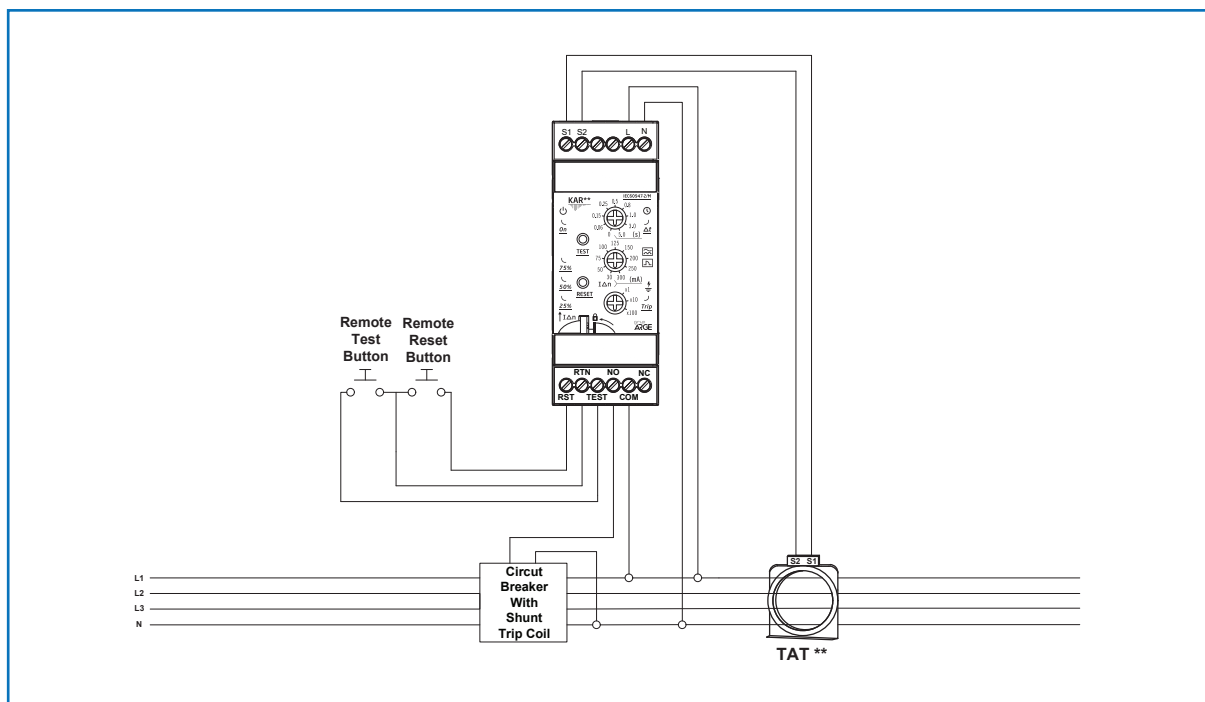
Figure 4: Toroidal Leakage Current Relay Connection Diagram
