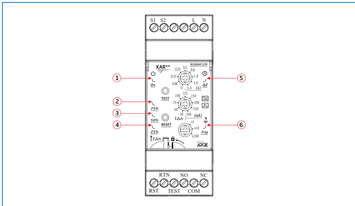
Figure 3: Front View of KAR01-KAR11 Leakage Current Relay
